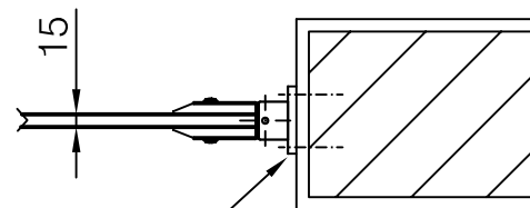
Stainless steel flat bar 80x8 mm
